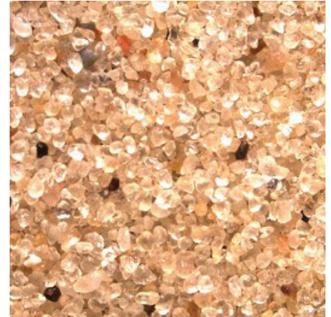
40/70-mesh standard frac sand suits technical and economic requirements for wells with normal closure stress.
